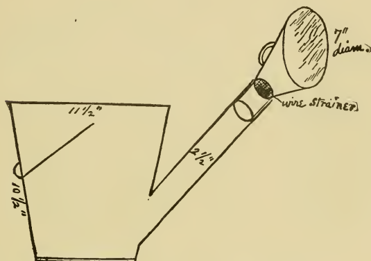
Modification of Stewart's Milk Pail.
